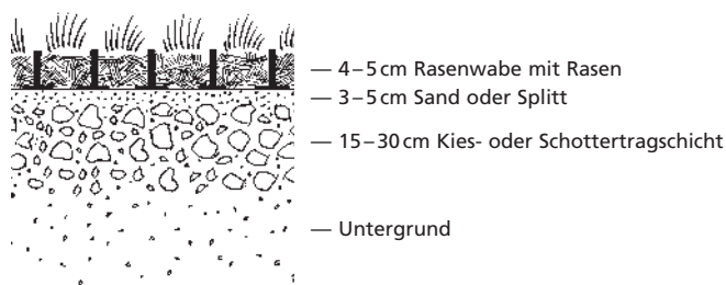
Rasenwabe
